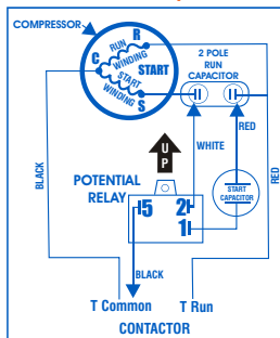
2 Pole Run Capacitor
