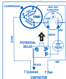
Dual Run Capacitor
