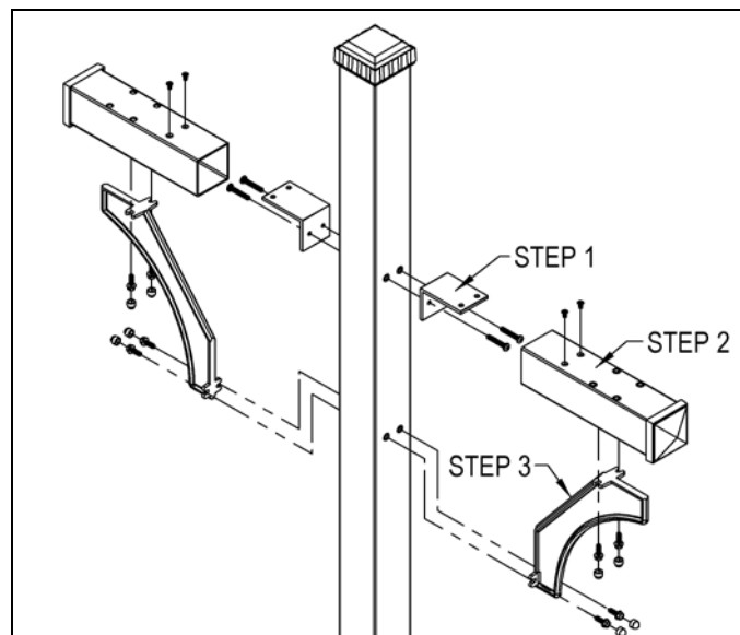
4372 Assembly
