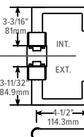
2190 WITH MW LEVER
