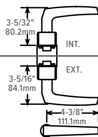
2190 WITH MJ LEVER
