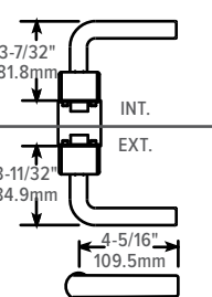
2190 WITH ME LEVER
