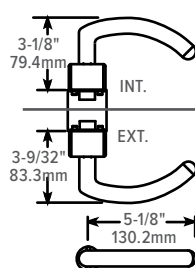
2190 WITH MG LEVER
