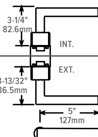
2190 WITH MI LEVER
