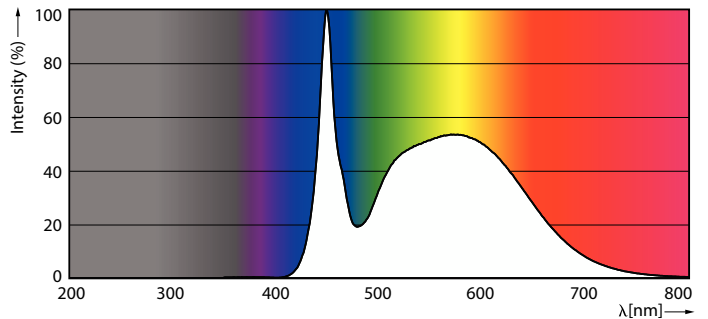
Spectral Power Distribution Colour - 14.5T8/COR/48-850/MF21/G 10/1
