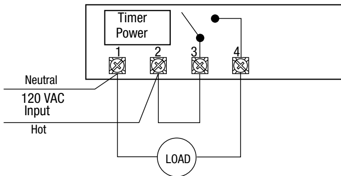
Example for 120 VAC input Model # EH10 SPST
