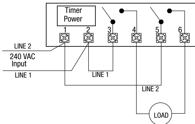
Example for 240 VAC input Model # EH40 DPST
