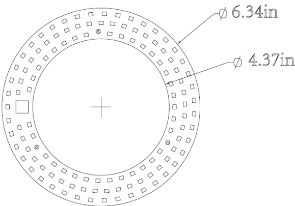
17W Ceiling Light, LED Circline Retrofit Kit, 3000K
